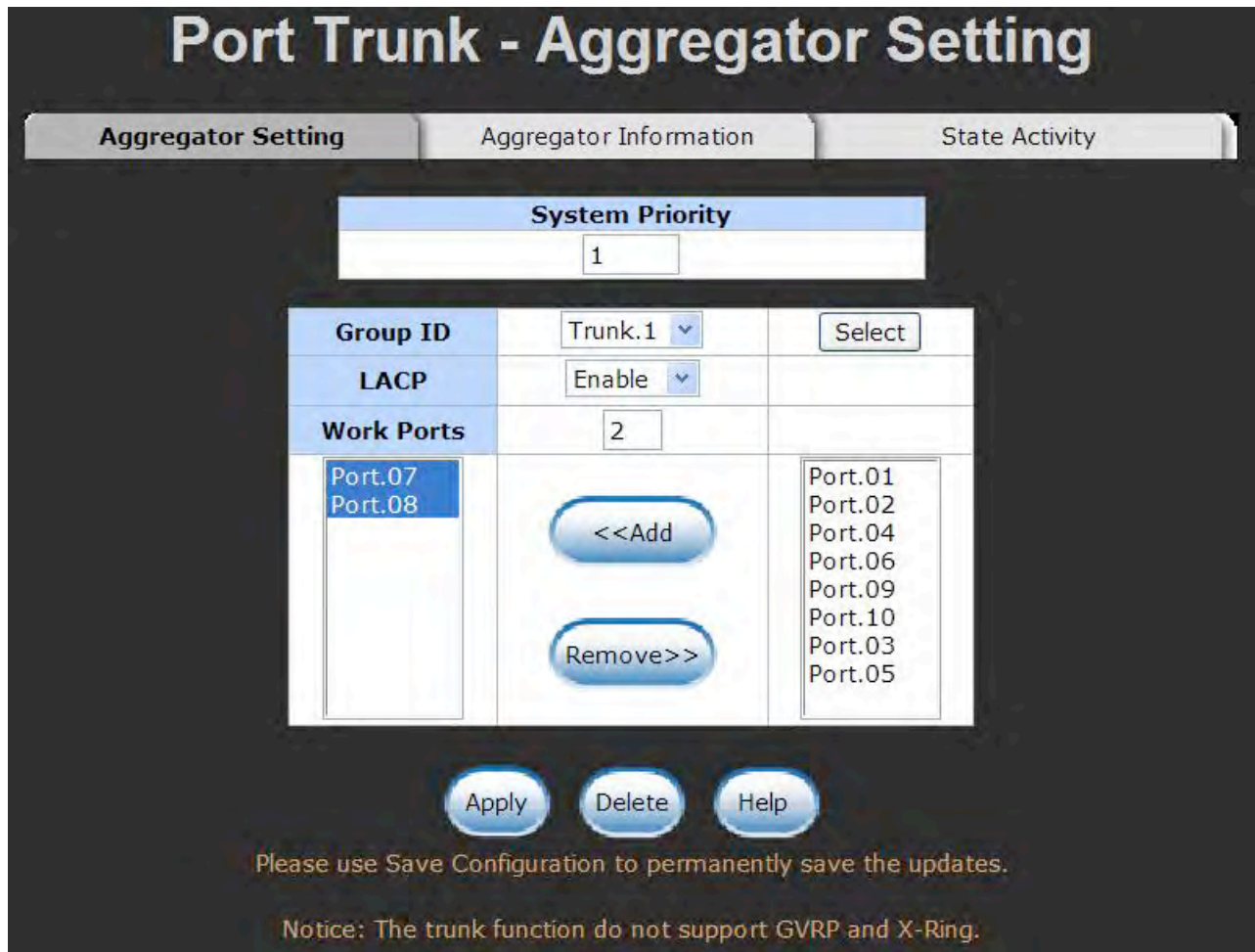
Switch 2 configuration interface
